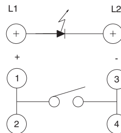
CIRCUIT
