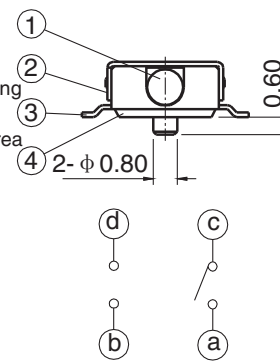
CIRCUIT DIAGRAM
