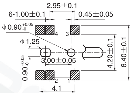
PCB LAND DIMENSION \phi \pm 0.05
