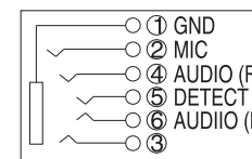
SCHMATIC
