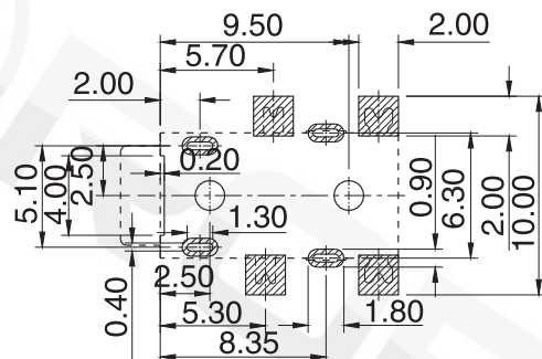
RECOMMENDED PCB LAYOUT TOP VIEW TOL:±0.05
