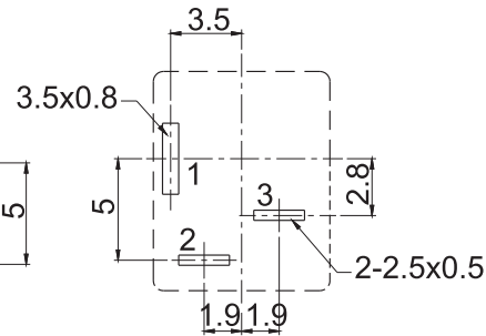
P.C.B Layout(Copper-side view)
