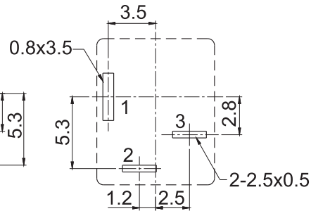
P.C.B Layout(Copper-side view)
