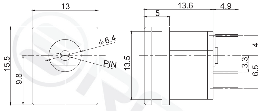
P.C.B Layout(Copper-side view)
