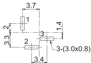
P.C.B Layout(Copper-side view)
