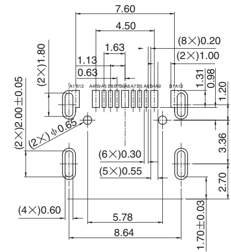
RECOMMEND PCB LAYOUT(TOLERANCE: ±0.05) (THICKNESS:0.8mm) SCALE:1:1
